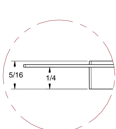
Detail A (Scale 3:2)
