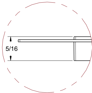
Detail A (Scale 3:2)
